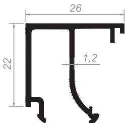
8mm CAM PROFİLİ 8mm GLAZING BEAD Kod/Code :OB-G01 Ağırlık/Weight:0,306 kg/m
