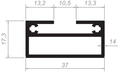
KASA PROFİLİ FRAME PROFILE
