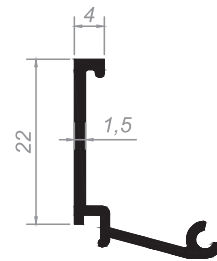
30mm CAM PROFİLİ 30mm GLAZING BEAD Kod/Code :OB-G05 Ağırlık/Weight:0,187 kg/m
