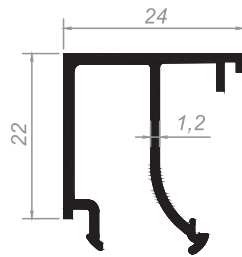
10mm CAM PROFİLİ 10mm GLAZING BEAD Kod/Code :OB-G04 Ağırlık/Weight:0,299 kg/m
